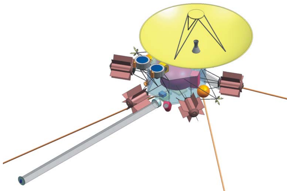
Figure 3. Innovative Interstellar Explorer based on radioisotope electric propulsion. The structure is dominated by six RPSs, the 3-m high-gain antenna, and the two ion engines. A 5-m magnetometer boom extends to the lower left; three mutually-orthogonal 25-m plasma wave antennas are partially visible.
