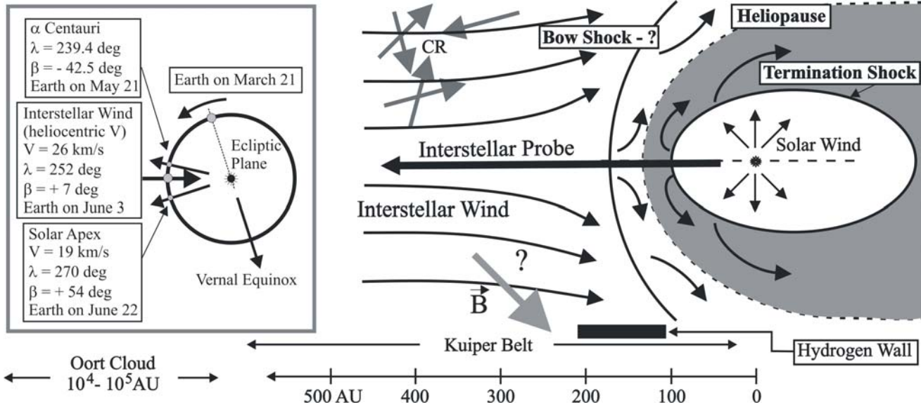
Figure 1. Sun's galactic neighborhood (right). Box (left) shows important directions in the ecliptic plane (interstellar wind vector, apex, \alpha -Centauri).
