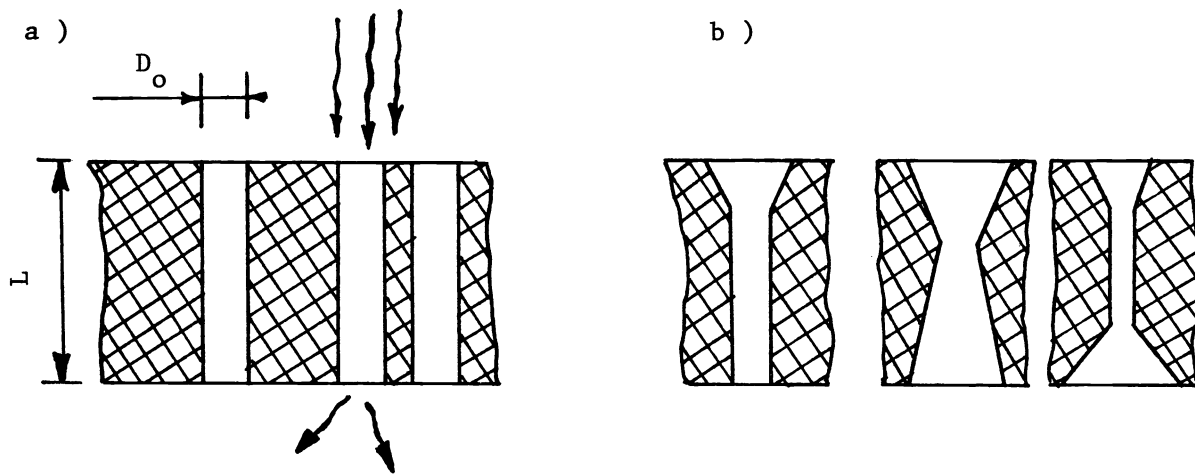
Fig.1. Films perforated by channels to filter the UV/EUV radiation. a ) straight parallel channels; b ) complex structure (funneled) channels.
